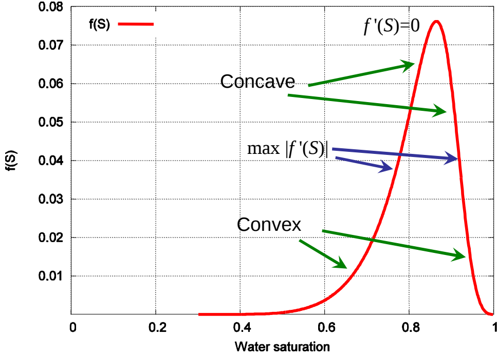
FIGURE 5. Plot of f(S) : normally the plot includes an interval of concavity between two intervals where the function is convex
