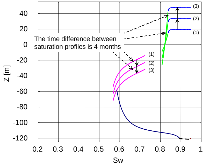
FIGURE 2. Evolution of water saturation profile in the plume. The origin, z = 0 , is associated with the center of the rarefaction wave at the top of the plume.
