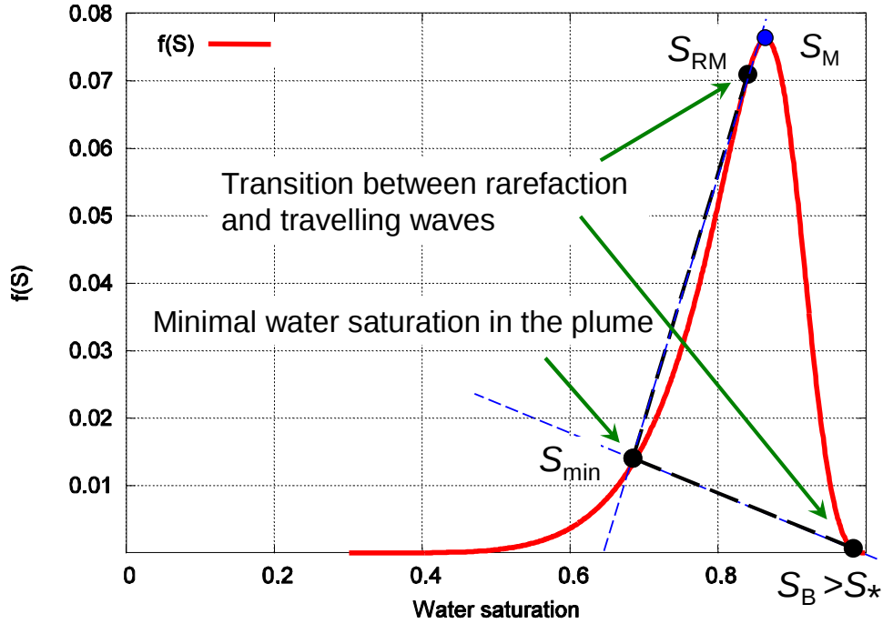
FIGURE 7. Saturations at the tail of rarefaction wave and the main part of the plume: the saturation at the transition point, S_{RM} is the tangential point between the plot of f(S) and a straight line passing through S_{min} . The transition saturation, S_B between the travelling and rarefaction waves at the bottom can be determined in a similar way.
