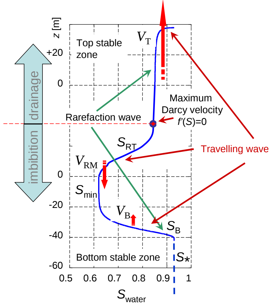
FIGURE 1. The top part of the plume is relatively “lean” with respect to the gas saturation, but propagates much faster than the bottom part saturated with gas.
