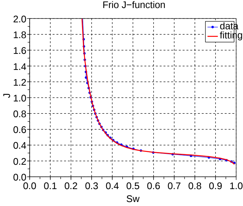
FIGURE 8. The blue curve with circle markers is the data, the red curve is the fitting curve. Fitting the plateau with the new parametrization
