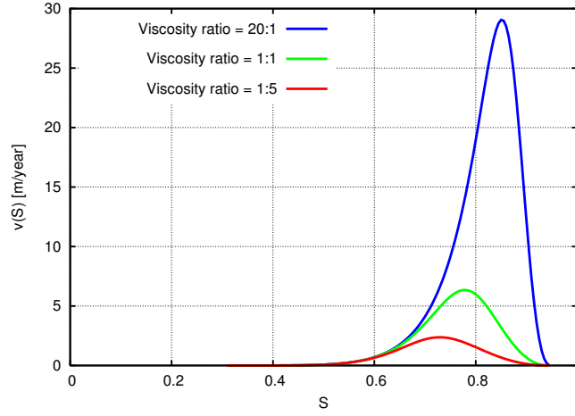
FIGURE 4. Plume migration velocity in m/year for three different viscosity ratios \mu_w : \mu_g .
