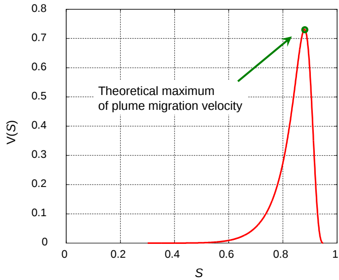
FIGURE 3. The maximum of the V(S) curve defines the theoretical maximum of the plume propagation velocity.
