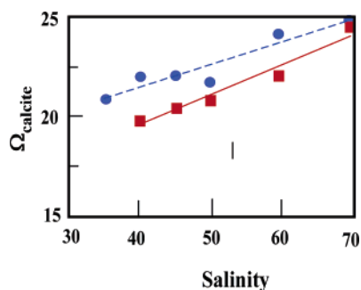
Figure 8. The supersaturation with respect to calcite ( \Omega_{\text{calcite}} ) necessary for pseudo-homogeneous nucleation of calcium carbonate from seawater at different salinities. Red line and symbols are at 25 °C, and blue line symbols are at 40 °C. Modified from ref 149, Copyright 1993, with permission from Elsevier.
