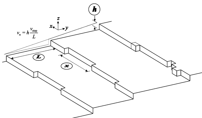
Figure 5. Schematic representation of parameters relating crystal growth and dissolution rate with bulk rate: surface step height, h ; kink spacing, x ; interstep spacing (terrace width), L .
