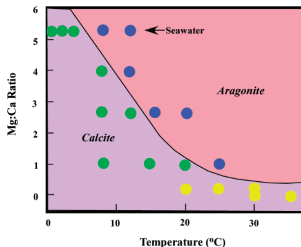
Figure 9. Influences of seawater Mg/Ca ratio and temperature on the nucleation of calcium carbonate from seawater. Blue circles are aragonite; yellow circles are calcite; green circles are initially calcite with aragonite overgrowths. Modified from ref 153 with permission. Copyright 1997 Geologic Society of America.
