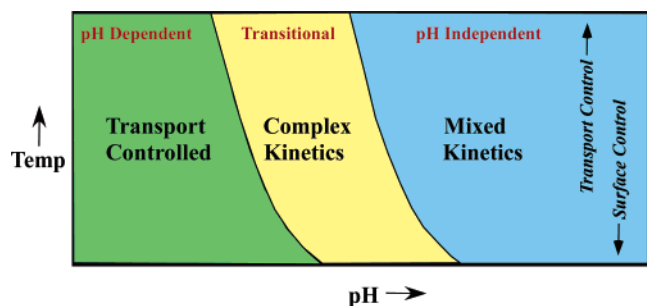
Figure 11. Summary diagram of relationship of transport versus surface-controlled dissolution based on the work of Sjöberg and Rickard. 162 Modified from ref 50, Copyright 2002 with permission from Elsevier.
