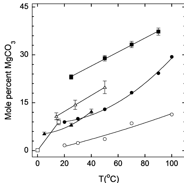
Figure 6. Variation of MgCO 3 content of magnesian calcite with temperature, precipitated in seawater or seawater-like solutions, adapted from Mucci 121 (see Mucci 121 for references to original data). Solid squares are CaCl 2 + MgCl 2 + NaCl; solid circles are seawater + Na 2 CO 3 + Ca(HCO 3 ) 2 ; open circles are seawater + Na 2 CO 3 ; open triangles are CaCl 2 + MgCl 2 + Na 2 CO 3 ; open squares are seawater + Na 2 CO 3 + aragonite seeds; solid triangles are seawater + calcite seeds. Reprinted from ref 121, Copyright 1987, with permission from Elsevier.
