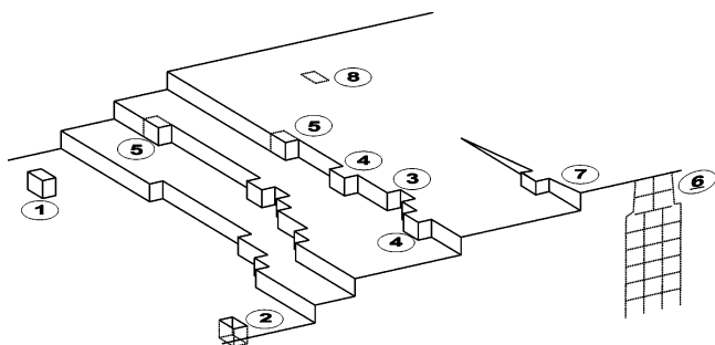
Figure 4. Schematic view of defects and specific sites on a crystal surface: (1) terrace adatom; (2) terrace vacancy; (3) step vacancy or “double” kink site; (4) step adatom; (5) single kink site; (6) outcropping edge dislocation; (7) outcropping screw dislocation; (8) imminent hole.
