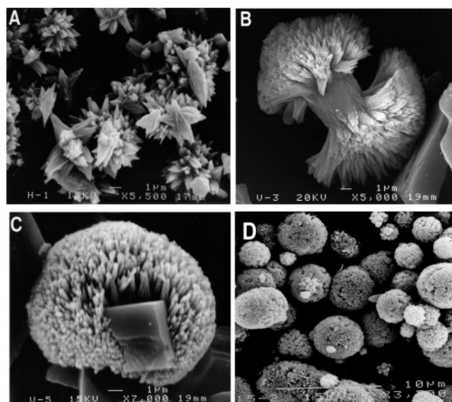
Figure 10. Scanning electron photomicrographs of calcium carbonate precipitated from seawater of various Mg/Ca ratios and temperatures: (A) aragonite with needle morphology from warm normal seawater; (B) aragonite with “broccoli” morphology from cold normal seawater; (C) aragonite needles growing on initially nucleated rhombohedral calcite for low Mg/Ca cold seawater; (D) radially fibrous aragonite sphere from 15 °C normal seawater. Panels A, B, and C reproduced from ref 153 with permission. Copyright 1997 Geologic Society of America. Panel D photo taken by J. Morse.
