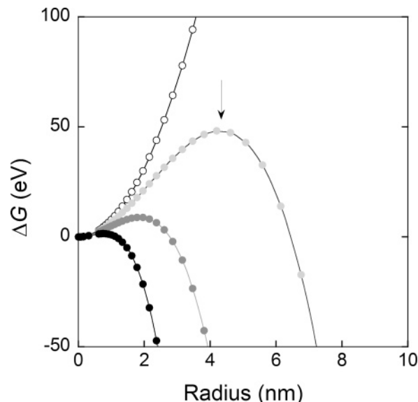
Figure 7. Variation of free energy ( \Delta G ) versus crystallite size (radius), computed as a function of increasing oversaturation ( \Delta\mu ) of the solution, using eqs 3.19 and 3.20. Open circles represent equilibrium condition, light gray circles represent \Omega = 2 (arrow indicates position of critical radius), dark gray circles represent \Omega = 5 , and black filled circles represent \Omega = 50 .
