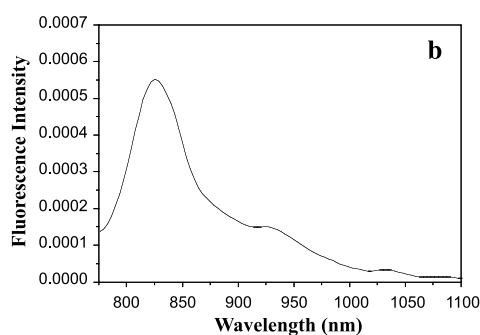
Figure 4: (a) Absorption and (b) fluorescence spectra of Cybesin in 20% aqueous DMSO. The fluorescence was excited by a 680 nm diode laser.
