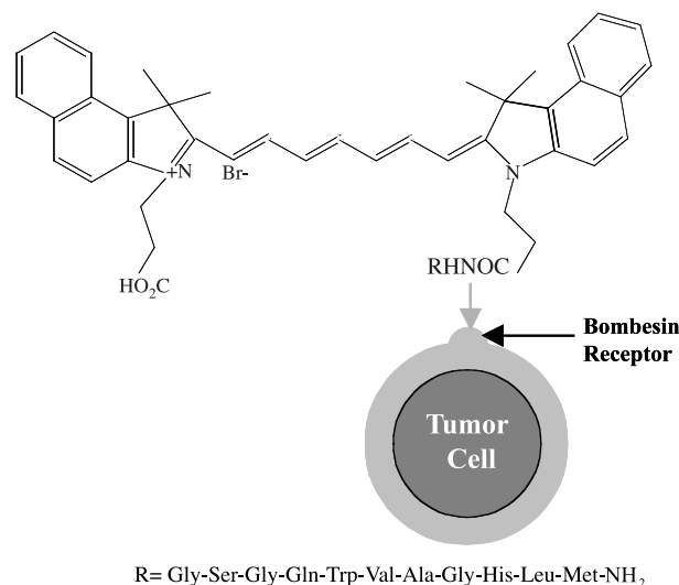
Figure 3: Molecular structure of the Cypate-Bombesin Peptide Analogue Conjugate (Cybesin), and schematic diagram of Cybesin targeting to the bombesin receptor on prostate tumor cells.
