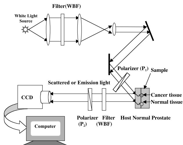
Figure 1: Schematic diagram of our spectral polarization imaging set-up. The structure of a sandwiched prostate cancerous-and-normal tissue sample is schematically shown in the sample position.
