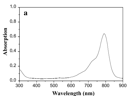
Figure 4: (a) Absorption and (b) fluorescence spectra of Cybesin in 20% aqueous DMSO. The fluorescence was excited by a 680 nm diode laser.
