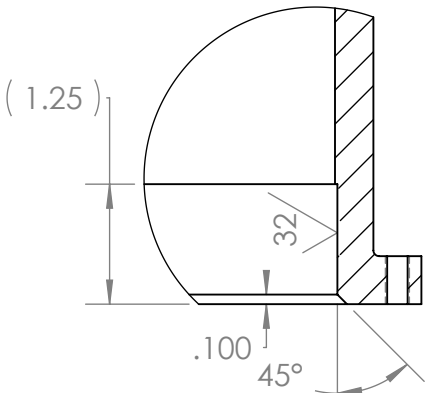
DETAIL H SCALE 1 : 2 Both Ends
