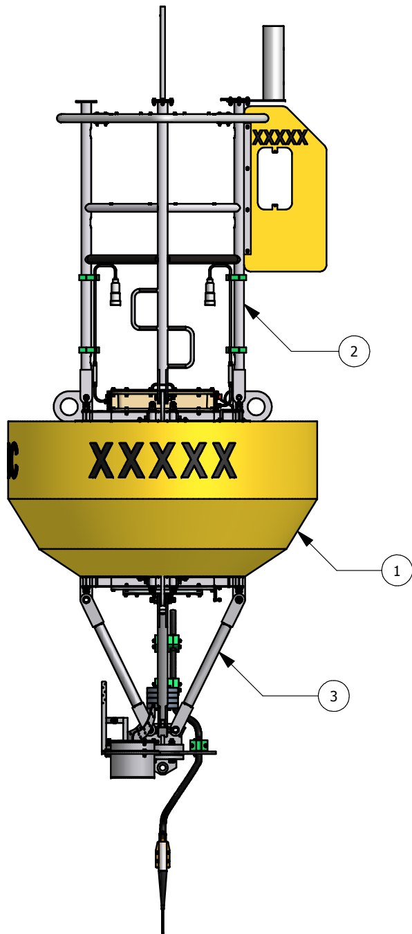
SIDE VIEW (270 DEGREES)
