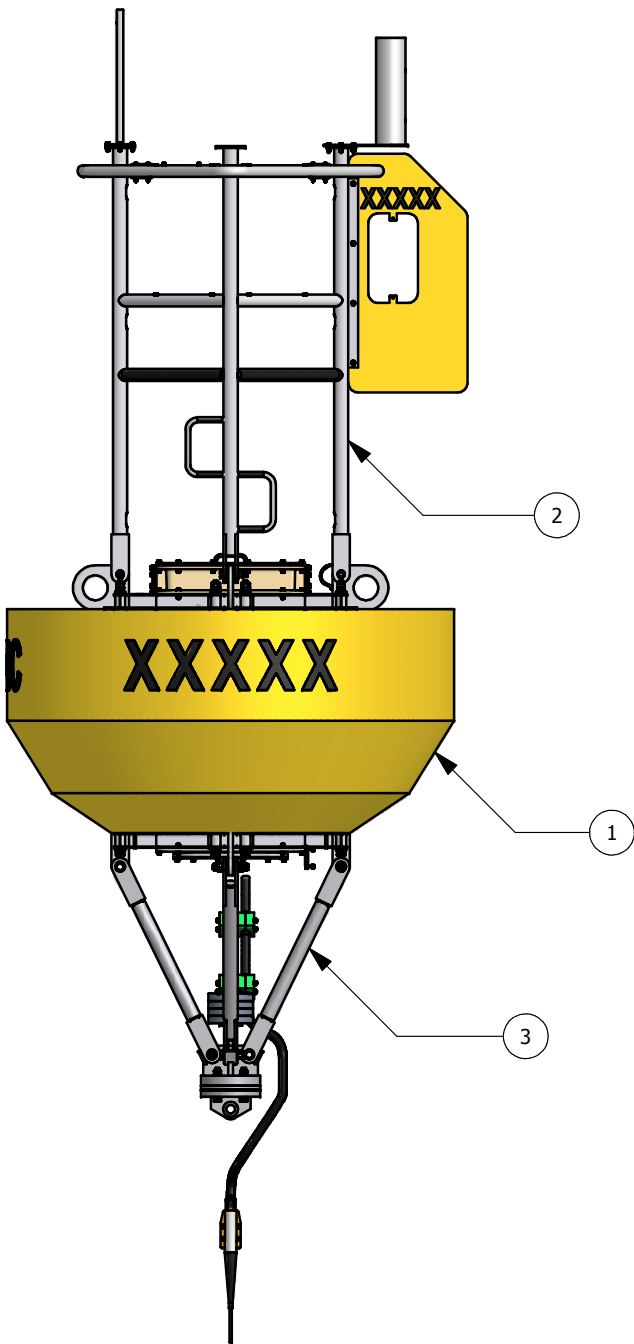
SIDE VIEW (270 DEGREES)
