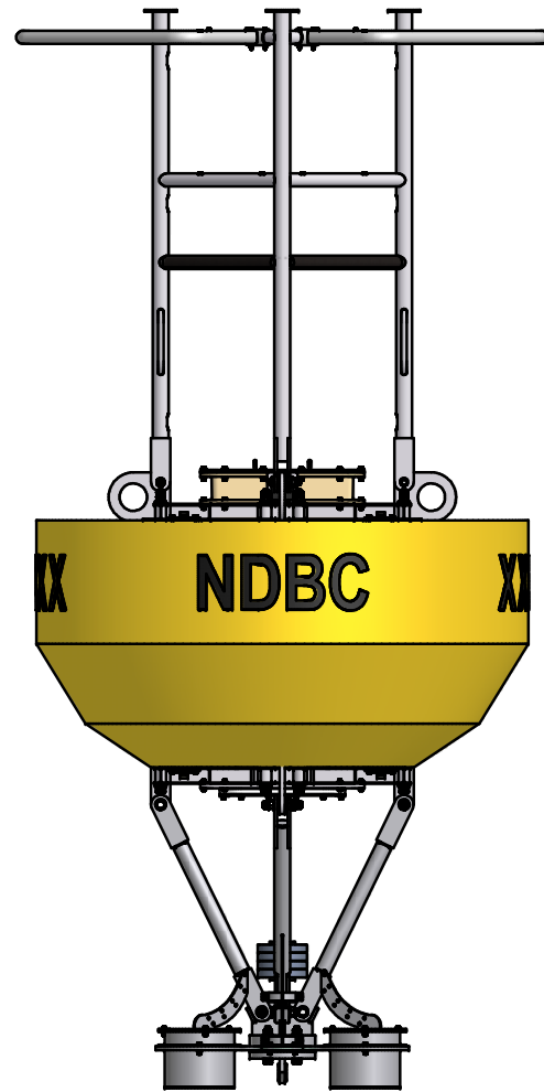
FRONT VIEW (0 DEGREES)
