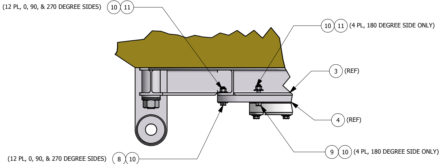
DETAIL D
