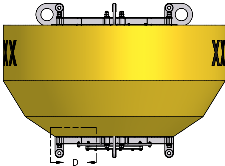
BACK VIEW (180 DEGREES) LOWER WELL ASSY. INSTL.
