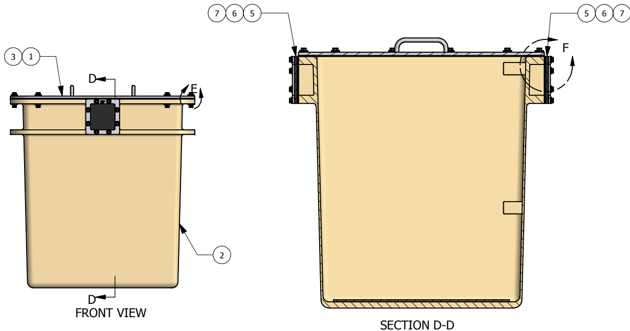
UPPER WELL ASSEMBLY -002 EMPTY CONFIGURATION
