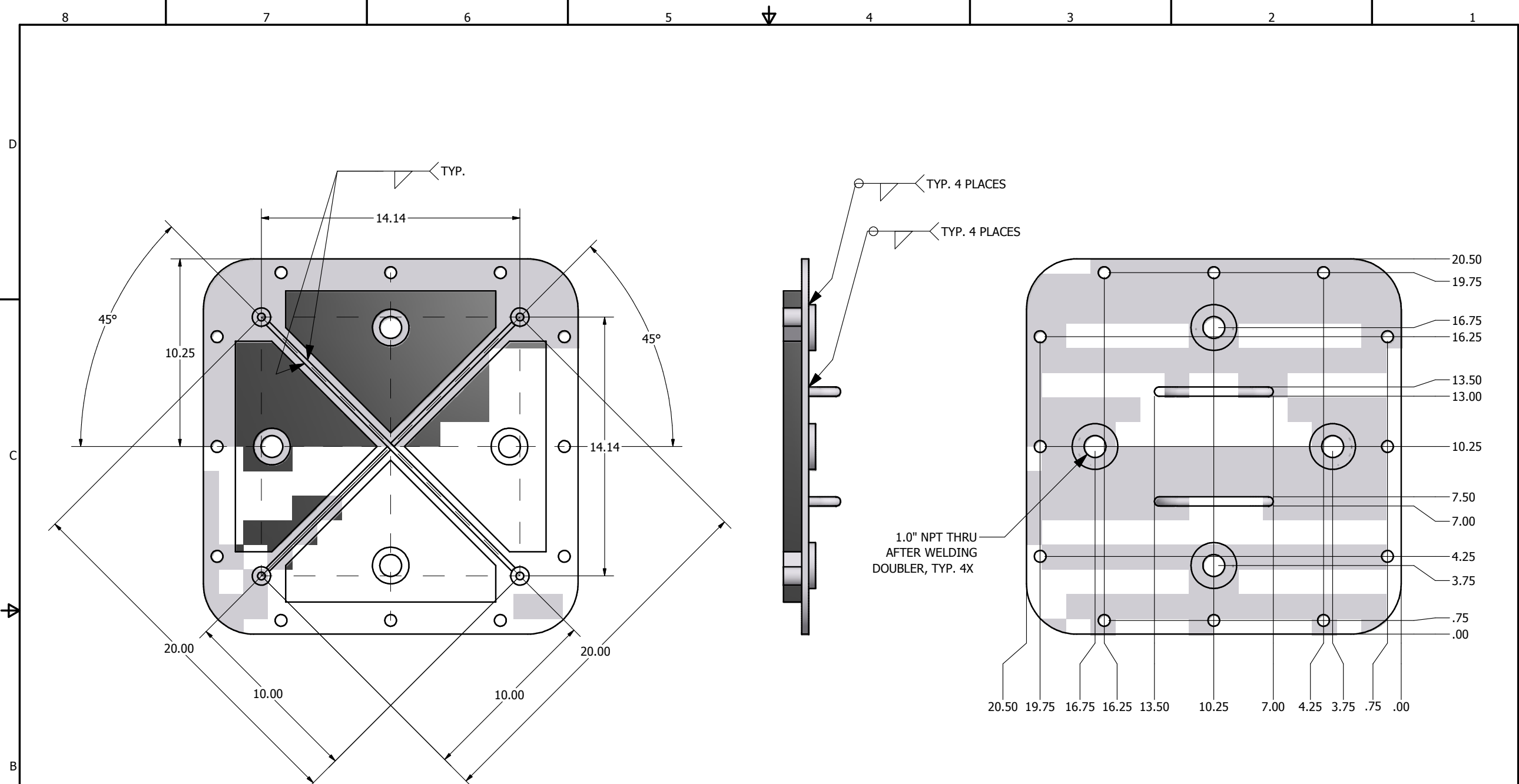
BOTTOM FABRICATION VIEW
