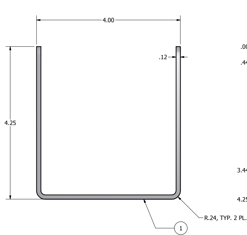
SIDE VIEW 1
