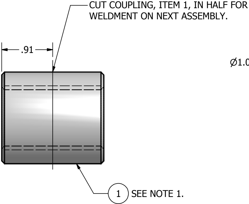
WHOLE COUPLER SIDE VIEW
