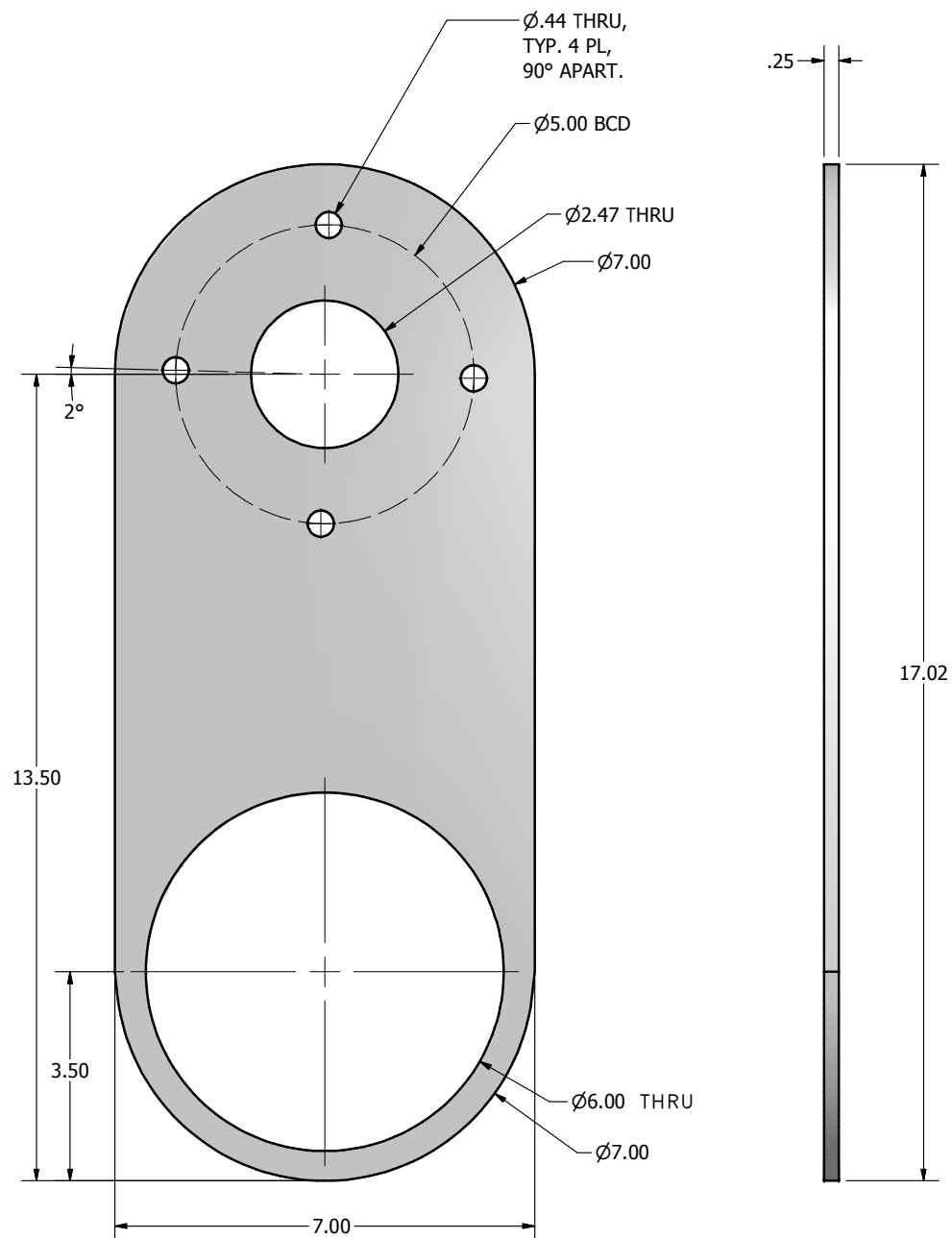
PLATE SIDE VIEW
