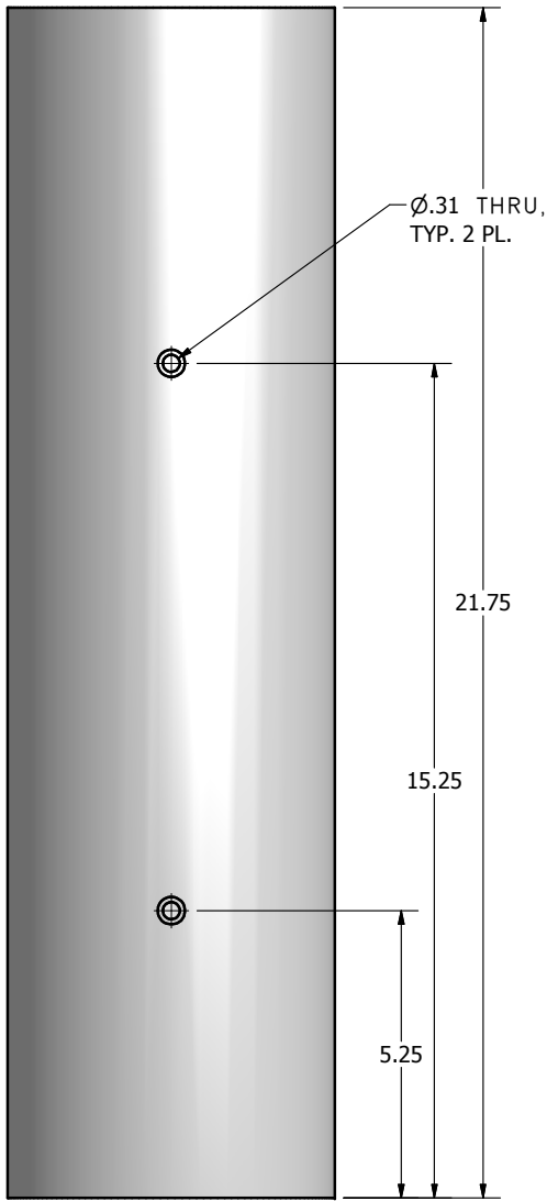
TUBE FRONT VIEW
