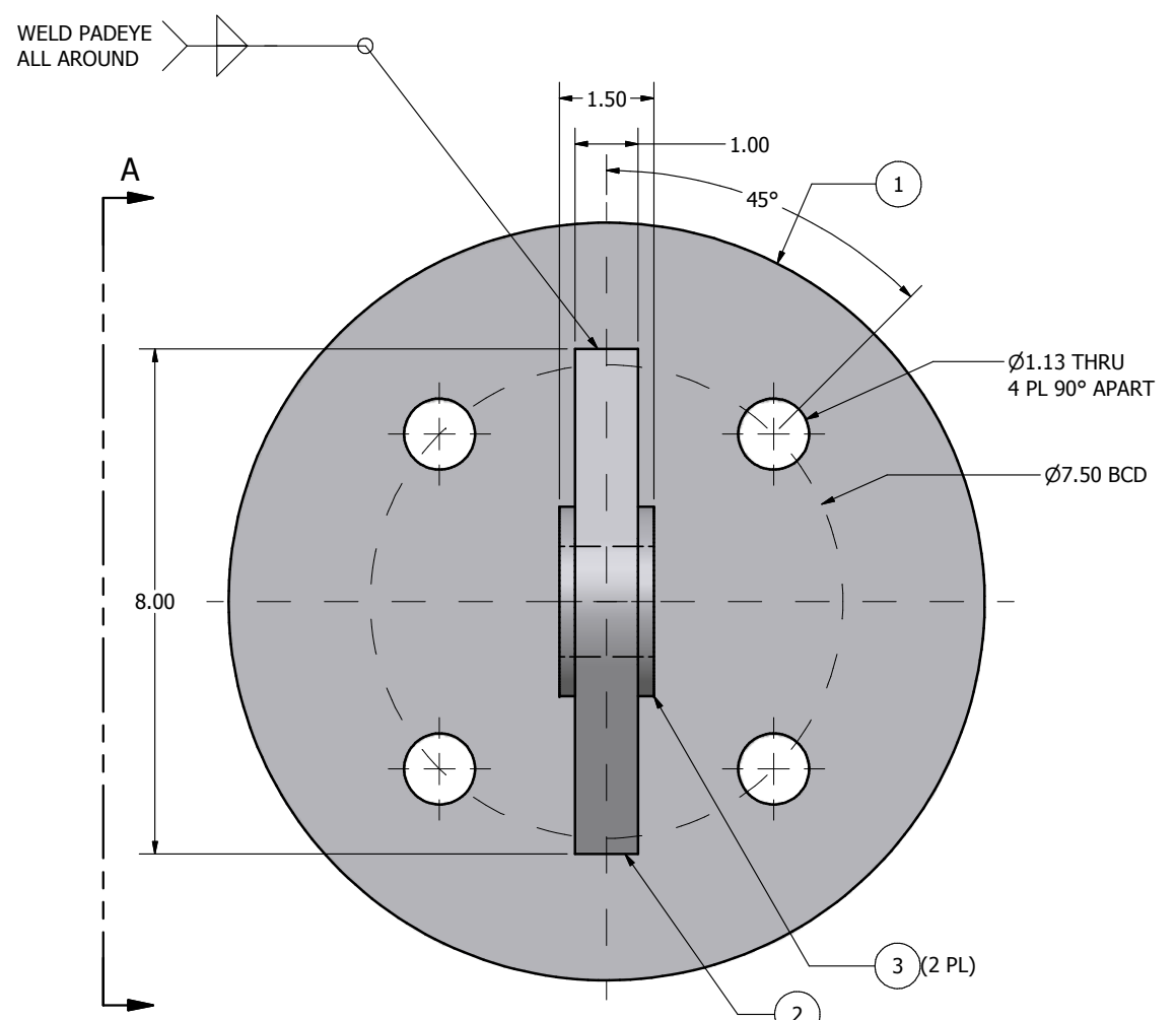
BOTTOM VIEW
