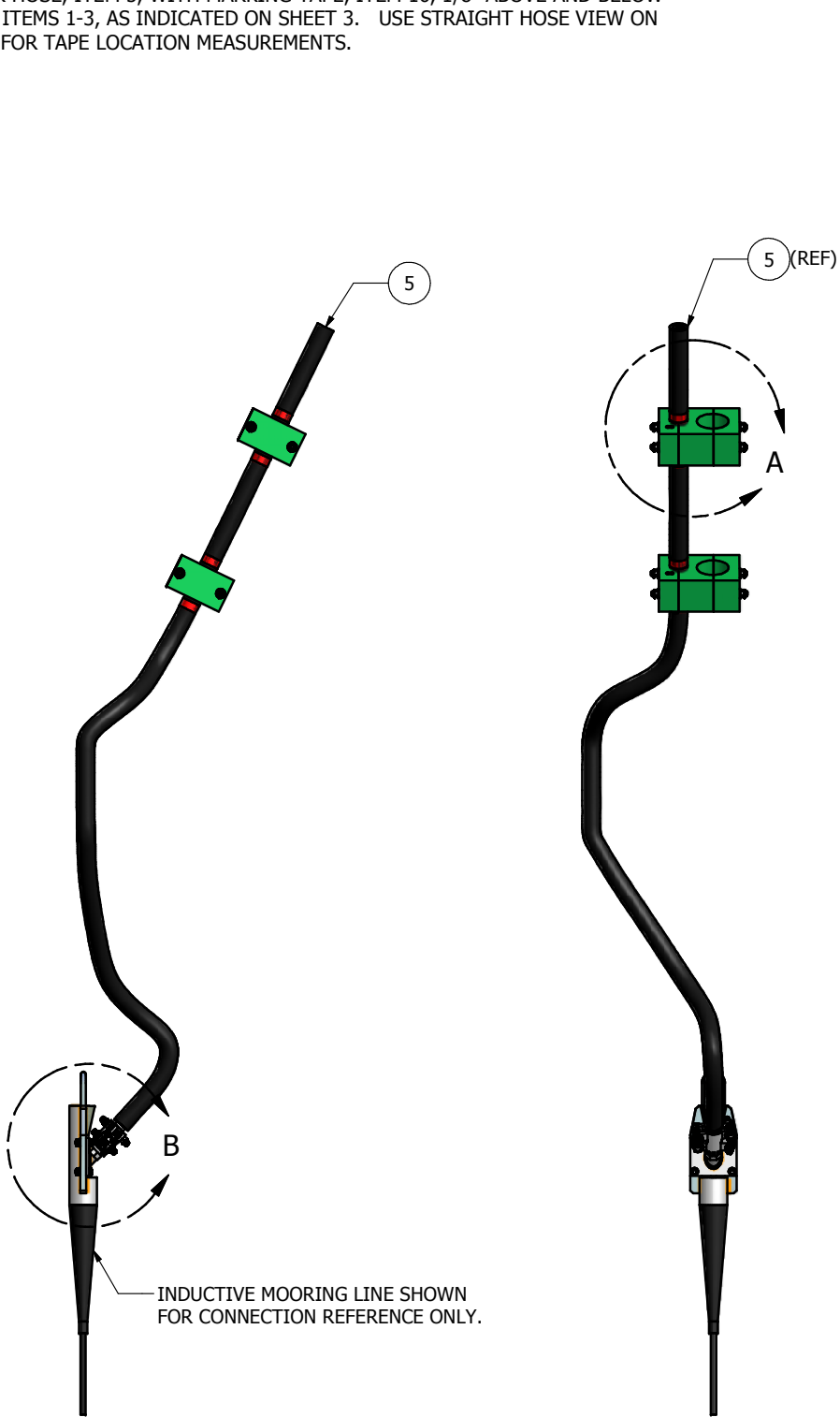
FRONT VIEW
