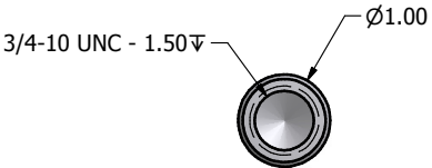
SUPPORT ROD TOP VIEW
