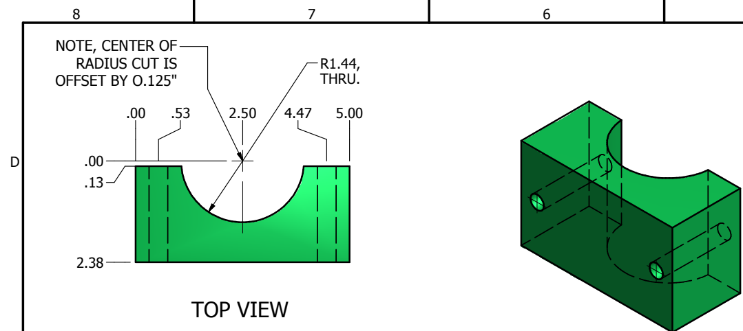
ISOMETRIC VIEW
