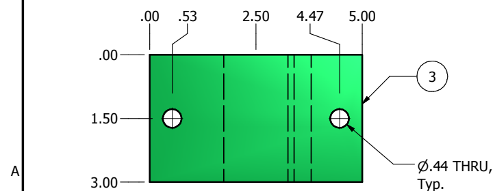
FRONT VIEW
