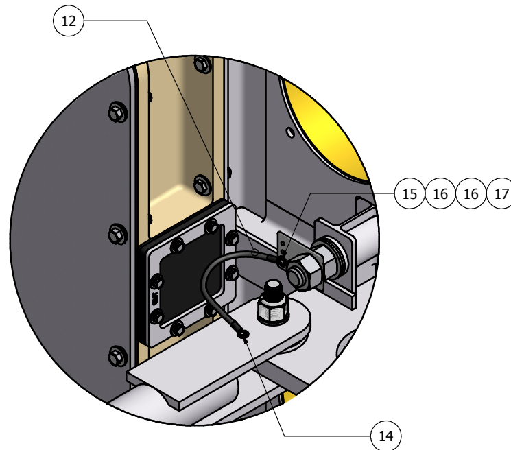
DETAIL F GROUND WIRE INSTALLATION
