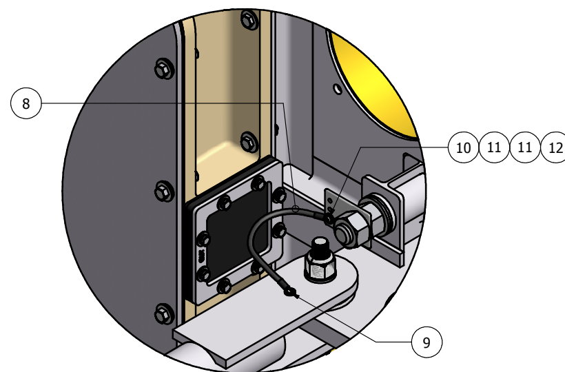
DETAIL J GROUND WIRE INSTALLATION
