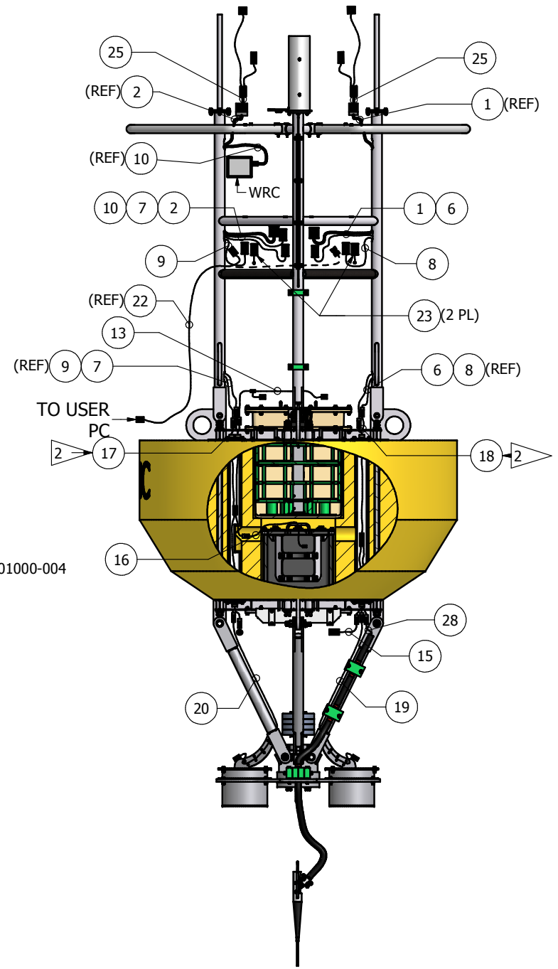
SIDE VIEW (270°) 2.3 METER STANDARD BUOY EXTERNAL CABLE INSTALLATION -004 WEATHER/DART CONFIGURATION (WEAH/DART)
