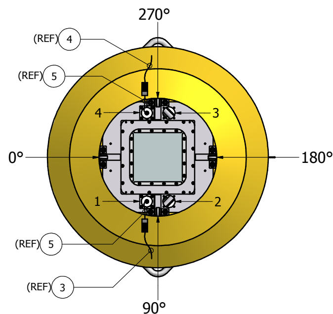
VIEW I-I FROM SHT. 5 BRIDLE REMOVED
