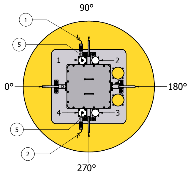
VIEW H-H FROM SHT. 5 TOWER REMOVED
