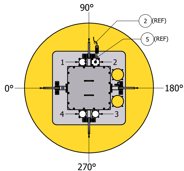
VIEW D-D FROM SHT. 3 TOWER REMOVED
