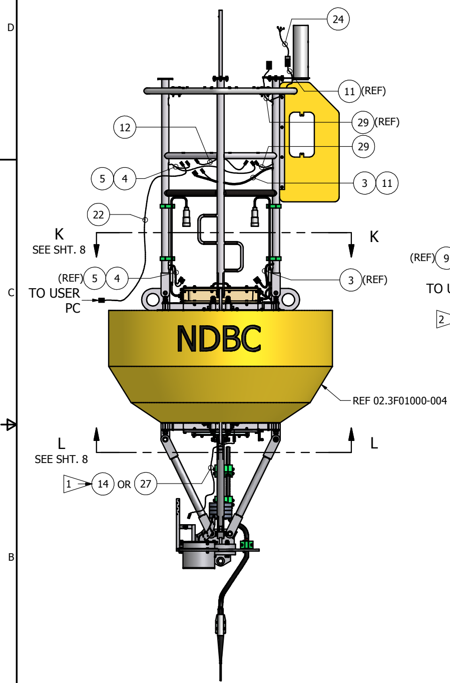
SIDE VIEW (270°) 2.3 METER STANDARD BUOY EXTERNAL CABLE INSTALLATION -004 WEATHER/DART CONFIGURATION (WEAH/DART)
