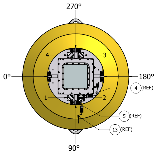
VIEW E-E FROM SHT. 3 BRIDLE REMOVED
