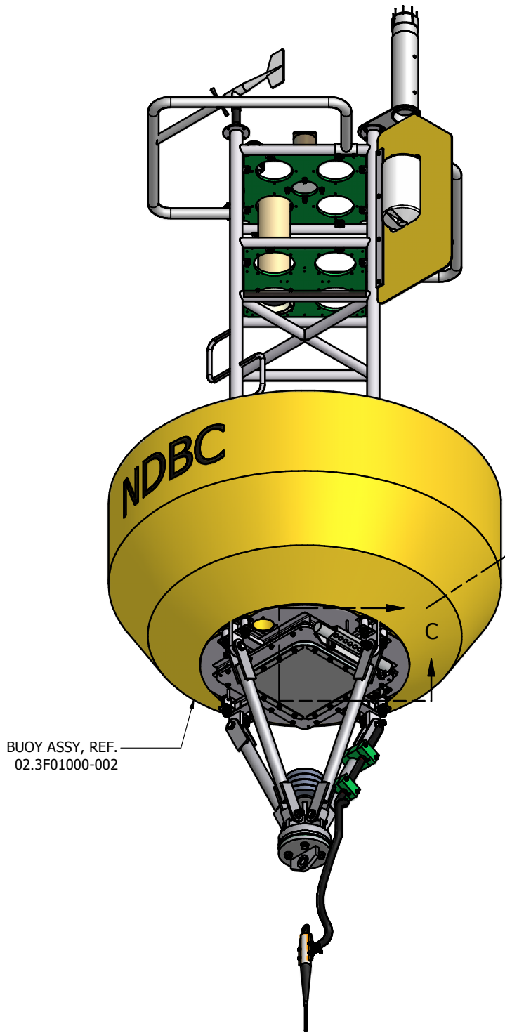
ISOMETRIC VIEW
