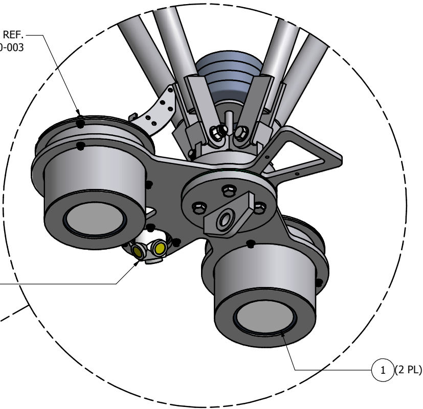
DETAIL D TRANSDUCER & SCM INSTALLATION
