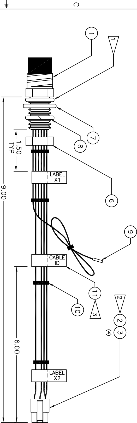
USER PORT PAYLOAD CABLE ASSEMBLY -001
