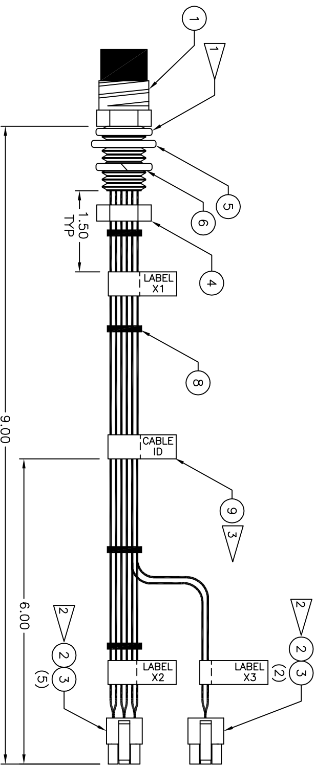
SOLAR RADIATION / RAIN PAYLOAD CABLE ASSEMBLY -002
