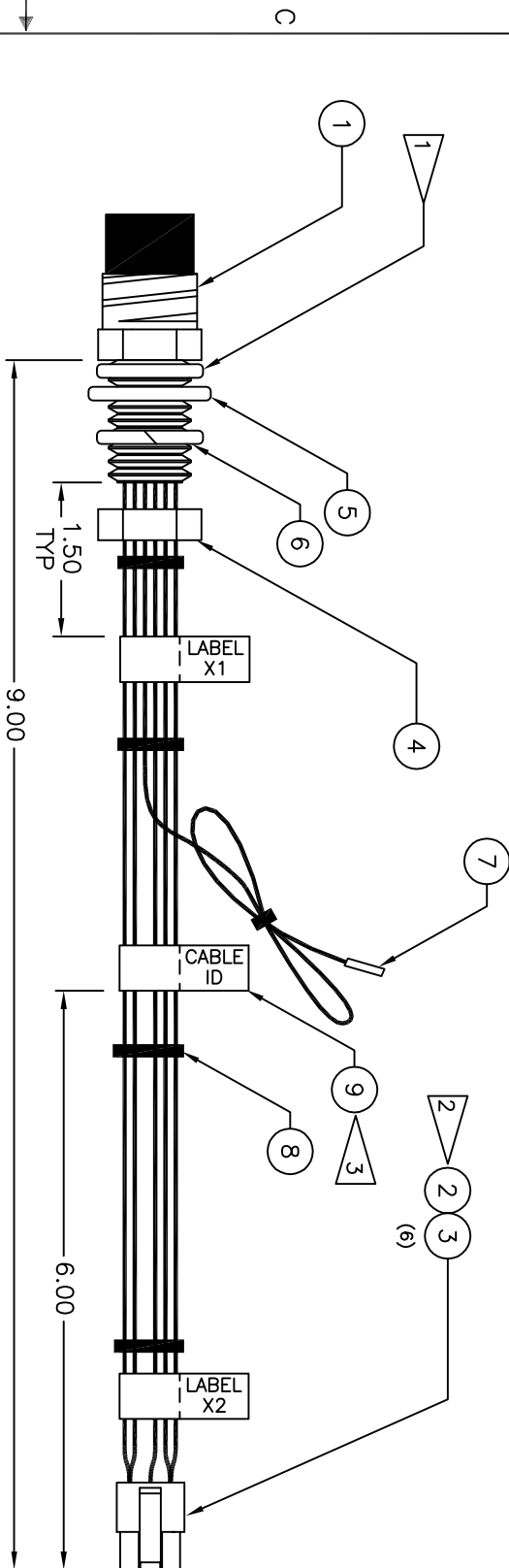
SIO1 PORT PAYLOAD CABLE ASSEMBLY -001
