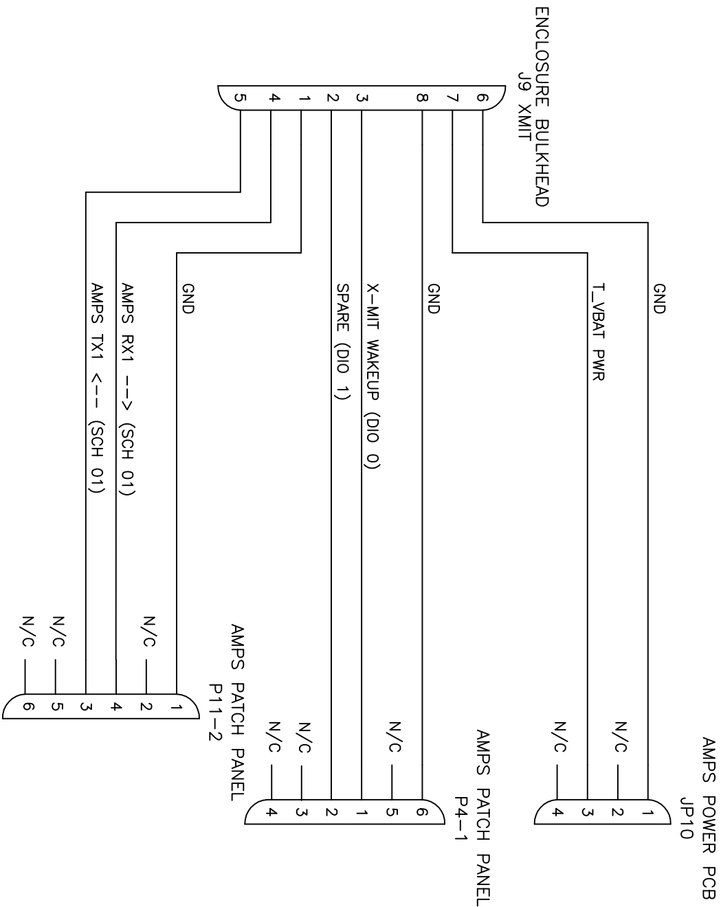
GOES INTERFACE PAYLOAD CABLE WIRING -001
