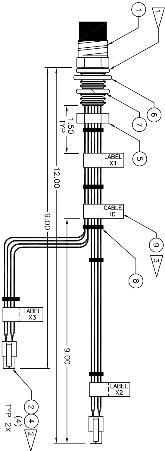
SUB-SURFACE INTERFACE PAYLOAD CABLE ASSEMBLY -002
