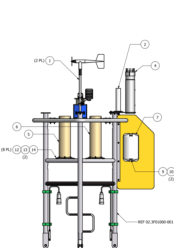
SIDE VIEW (270°) HULL & BRIDLE REMOVED
