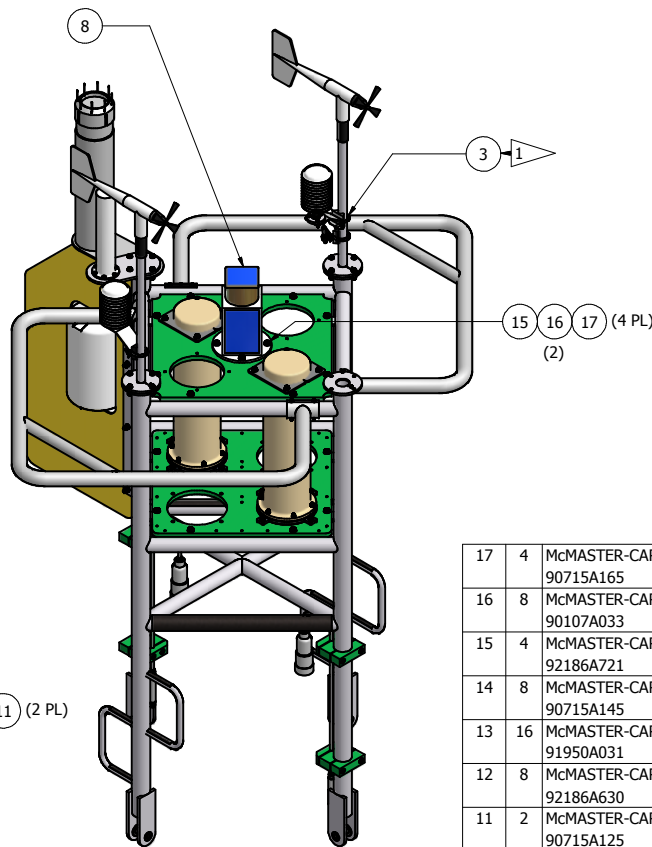
ISOMETRIC VIEW HULL & BRIDLE REMOVED
