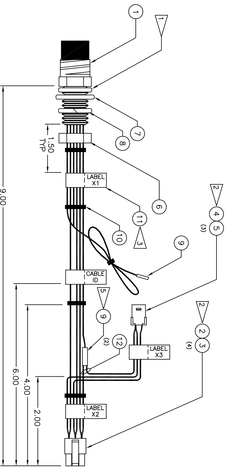
USER PORT PAYLOAD CABLE ASSEMBLY -002
