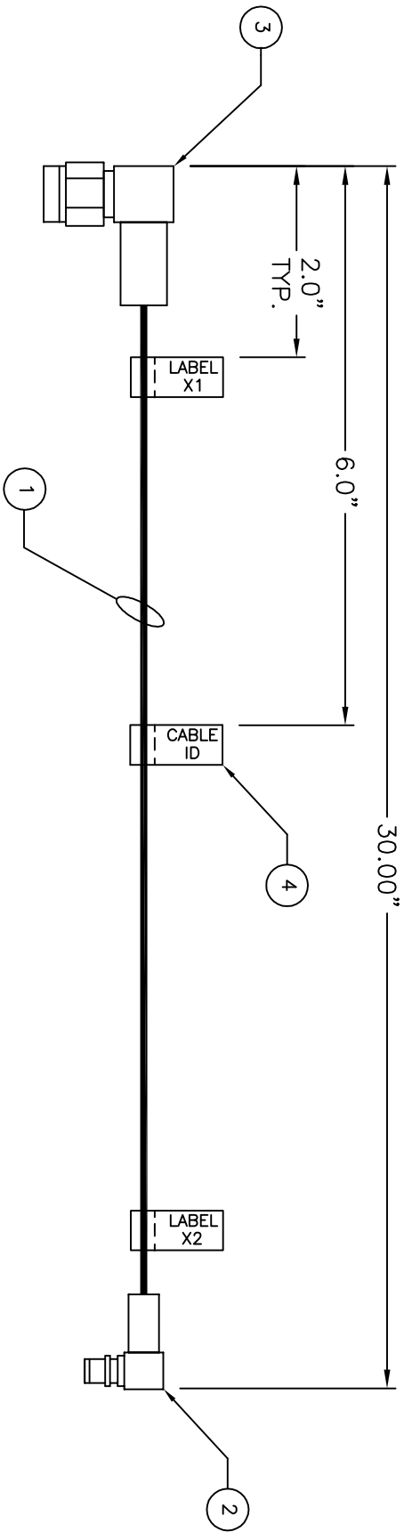
GPS COAX PAYLOAD CABLE ASSEMBLY -001
