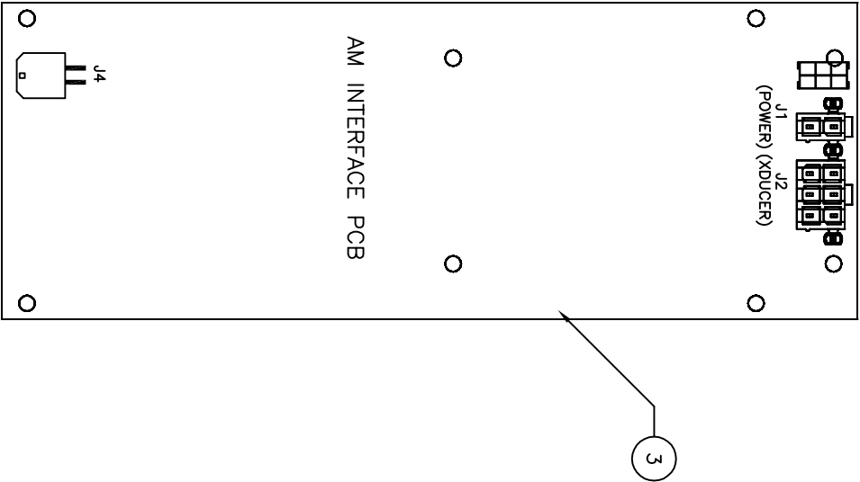
DETAIL B AM INTERFACE PCB 1/2
