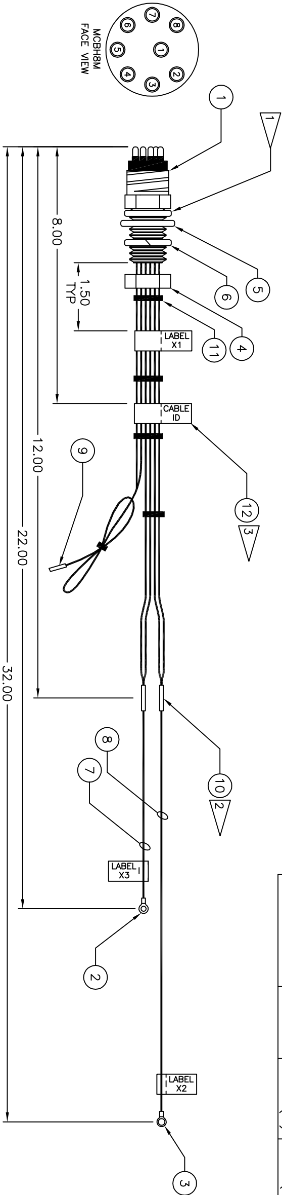
INPUT POWER UNIT CABLE WIRING -001
