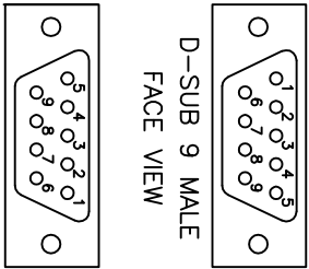
D-SUB 9 MALE WIRE ENTRY VIEW
