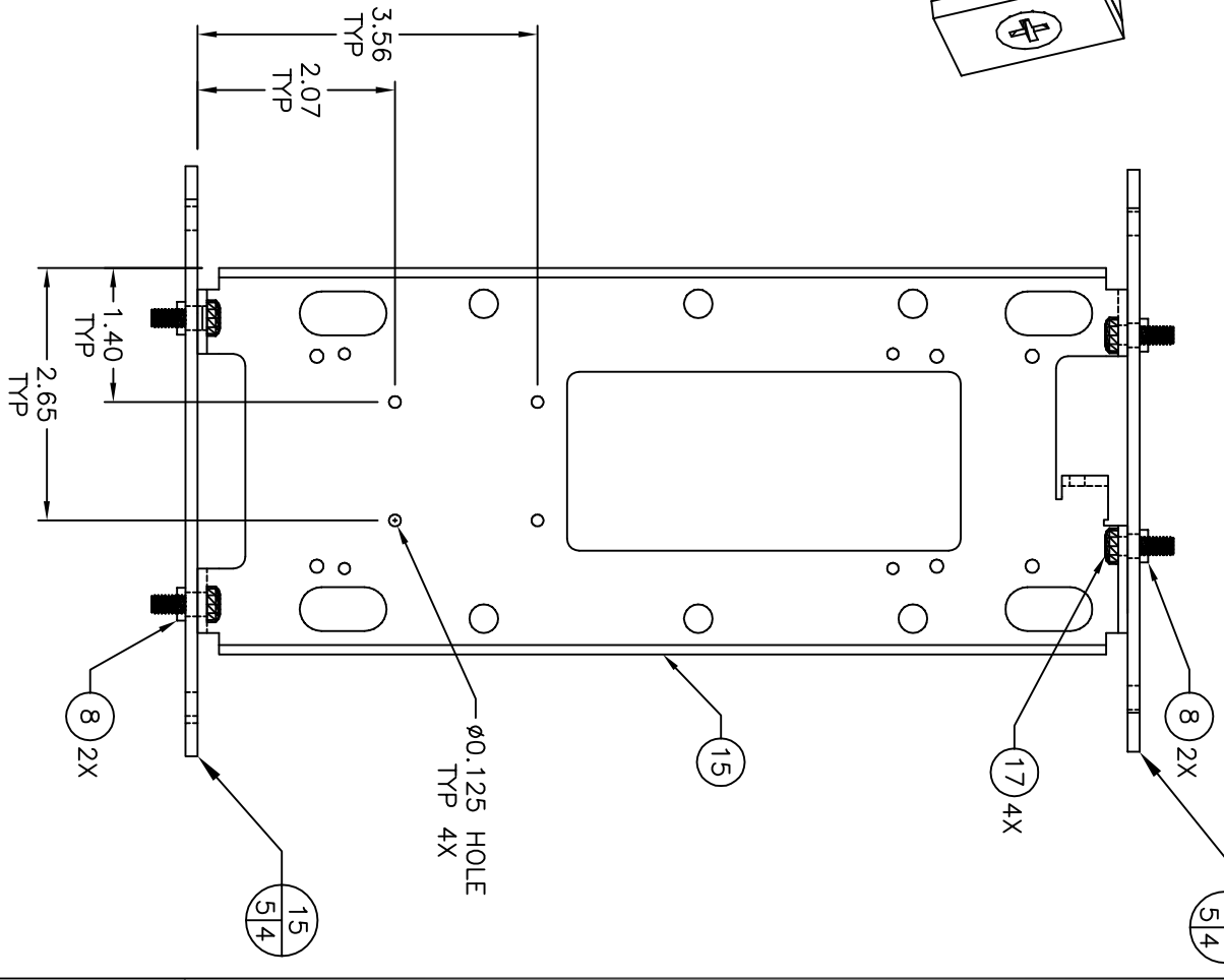
DETAIL 14
