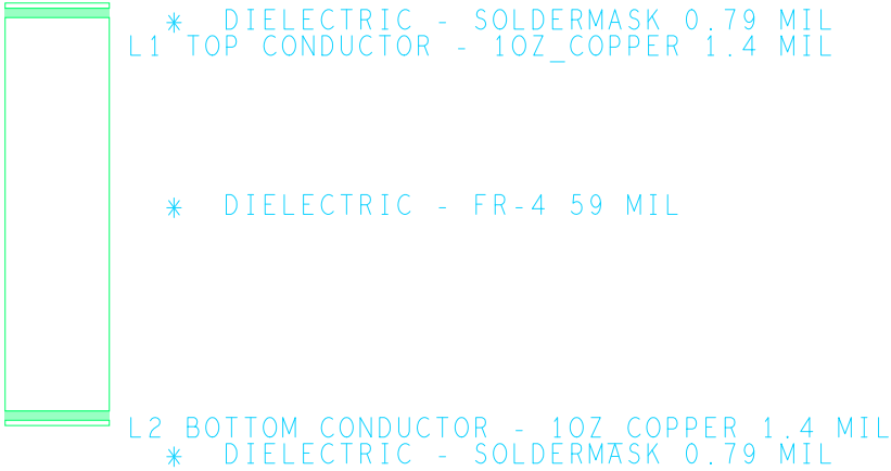
DESIGN CROSS SECTION CHART TOTAL THICKNESS 63.37 MIL
