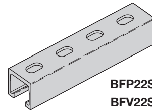
BFP22H1 7/8 BFV22H1 7/8 9/16" (14.3) holes 17/8" (47.6) on centers
