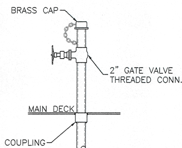
DETAIL 3-E TYPICAL POTABLE WATER FILLING CONNECTION SCALE: 1" = 1'-0"
