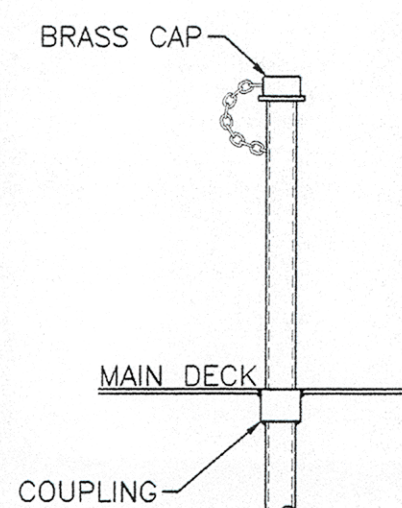
DETAIL 3-F TYPICAL FILLING CONNECTION SCALE: 1" = 1'-0"
