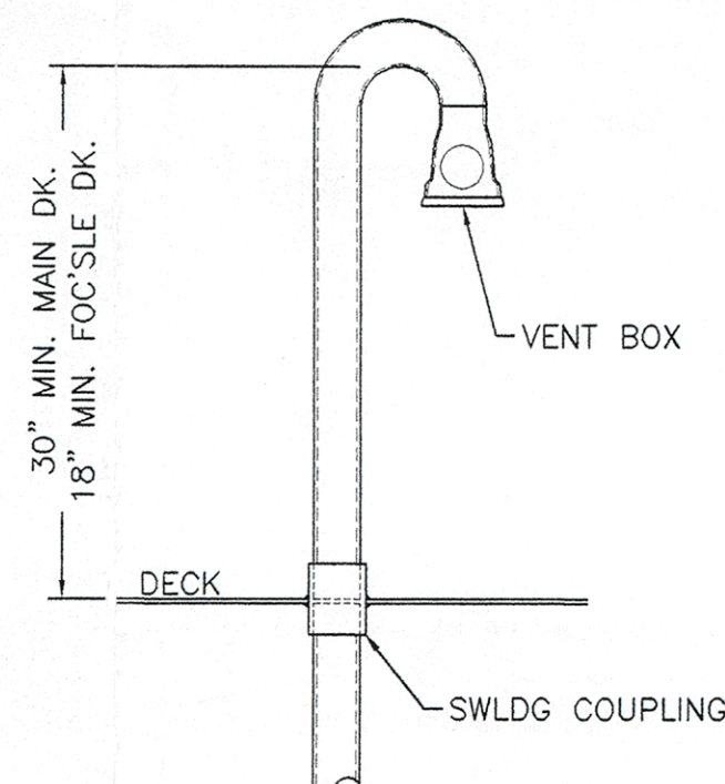
DETAIL 2-E TYPICAL REMOTE PENETRATION VENT DETAILS SCALE: 1" = 1'-0"
