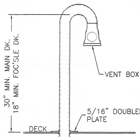
DETAIL 1-E TYPICAL LOCAL TANK PENETRATION VENT DETAILS SCALE: 1" = 1'-0"
