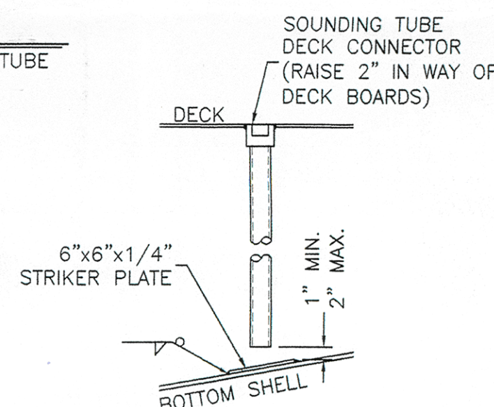
DETAIL 1-C TYPICAL SOUNDING TUBE SCALE: 1" = 1'-0"
