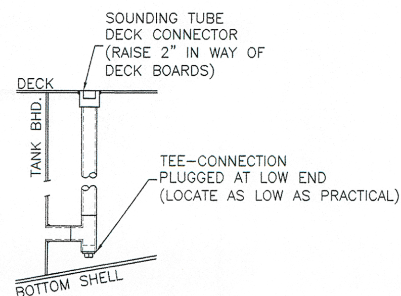
DETAIL 2-D TYPICAL REMOTE SOUNDING TUBE SCALE: 1" = 1'-0"
