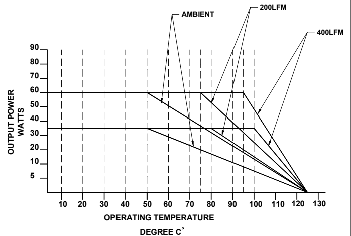
FIGURE 10B. Typical derating curves for Q75 PowerWatt series (For output power of 60W or less)
