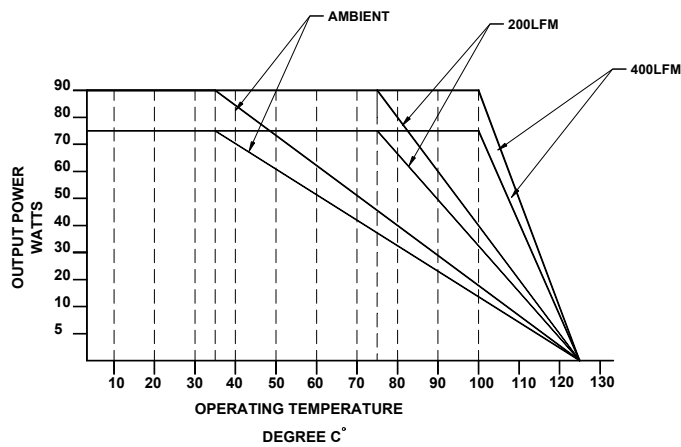
FIGURE 10A. Typical derating curves for Q75 PowerWatt series (For output power from 75W to 90W)
