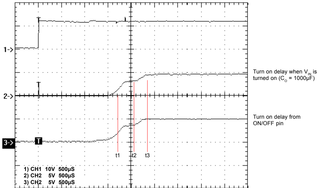
FIGURE 4. Turn on delays (Refer to Figure 3A)
