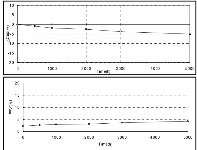
EEVEB2E470 (250V47 \mu F, \phi 16x21.5L)
