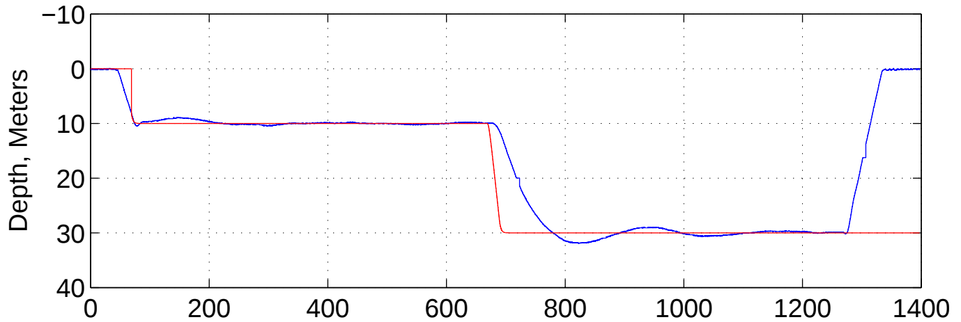
Depth: Red is Commanded, Measured is Blue, Data Set: 2004.337.02
