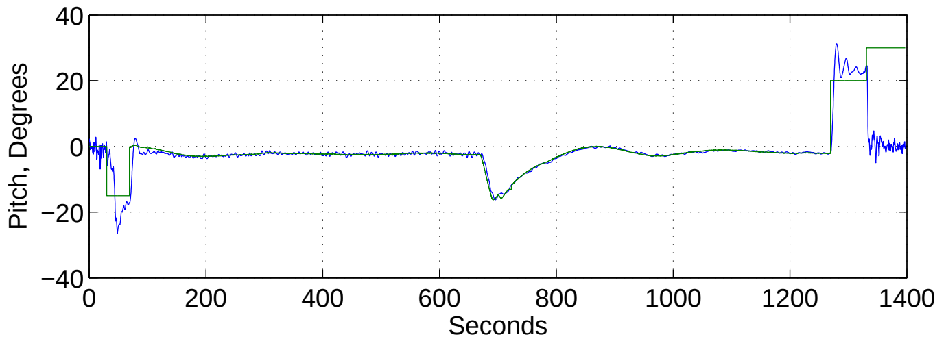
Vehicle Pitch: Commanded-Green; Measured-Blue
