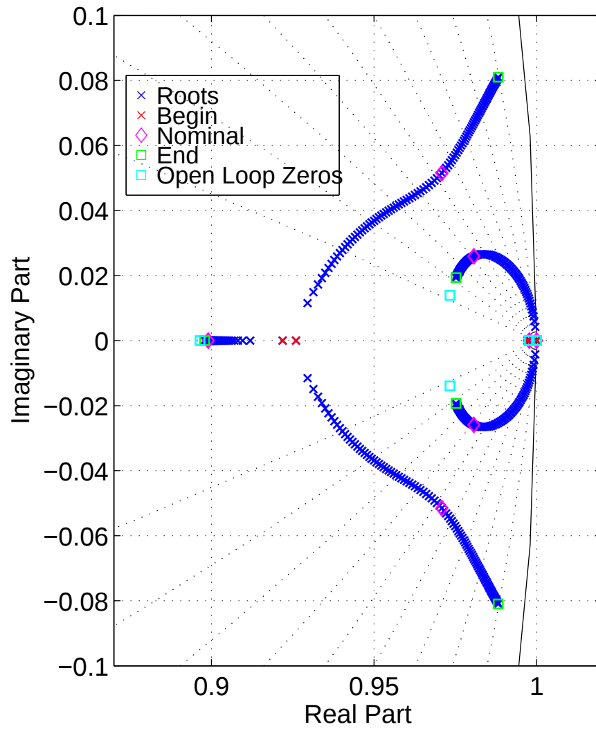
Pitch/Depth Root Locus on Actuator Gain at \delta_E
