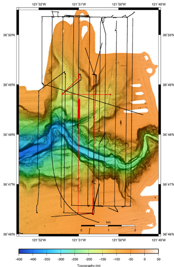
Figure 4. Location map of the Spring 2004 Mapping AUV sea tests. Subbottom profile data was collected along 140 km of tracklines across the upper Monterey Canyon. The red track shows the mission displayed in Figure 4. The thick red track is the location of the subbottom profile displayed in Figure 5.
