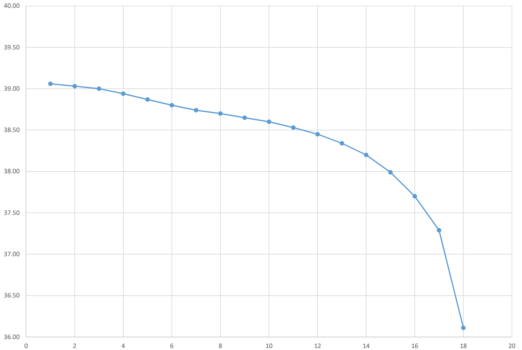
Dakota 36V/63Ah 4P Discharge at 50 Amps
