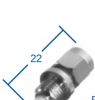
FIG. 13 RSA-3200, -1
