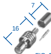
FIG. 6 RSB-4050-B, -B1, -1B
