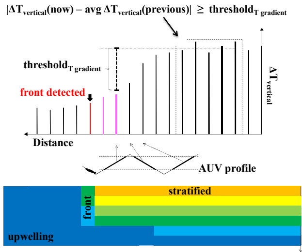
Fig. 8 A graphical representation of the upwelling front sampling algorithm employed by the CTD/Gulper AUV, with corresponding water types indicated below. The AUV accurately locates the front when detecting a sharp horizontal gradient of the vertical temperature difference \Delta T_{\text{vertical}} , and accordingly triggers water sampling. Modified from Y. Zhang et al. 2012.
