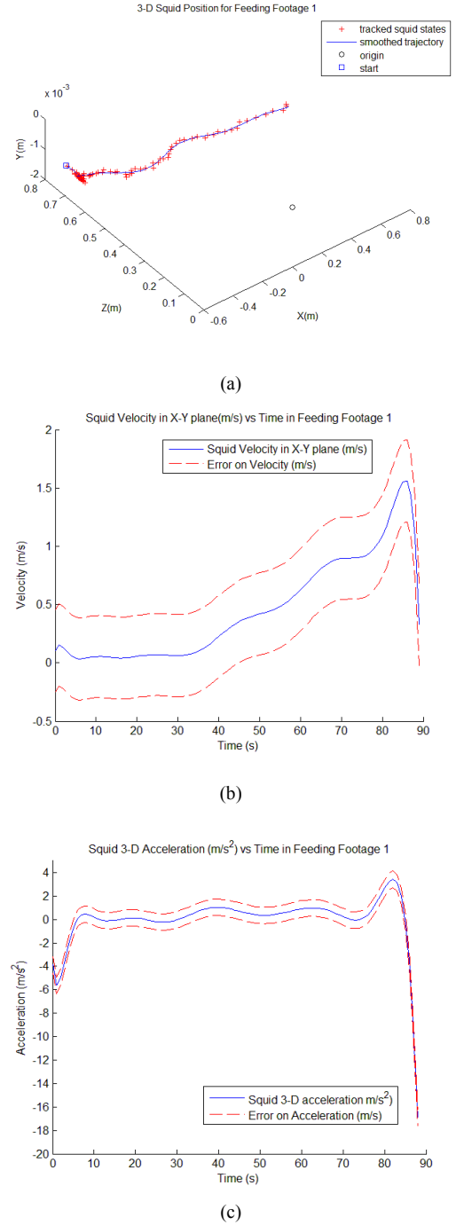
Fig. 9. Footage from Squid Feeding 1. Shown in (a) is the 3-D trajectory of squid with the ROV located at the origin. In (b), the smoothed velocity of squid within the x-y plane. In (c), the smoothed acceleration of squid is shown.
