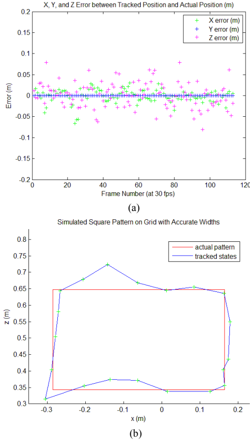
Fig. 8. Using accurate width dimensions. In (a), errors in x, y, and z direction in a truth test video. In (b), The red line is a simulated box pattern along a checked grid, and the blue line is the pattern estimated using the tracked x coordinates and width-to-z camera calibration.
