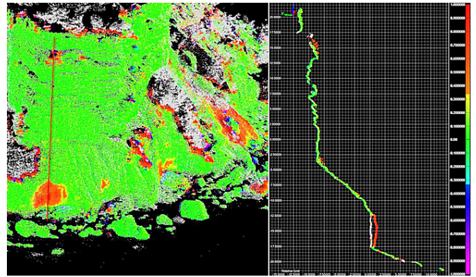
Fig. 10. Cliff meshes are subtracted to detect and quantify change (top view left; cross-section view, right). The mesh is colored to represent the magnitude of material loss.
