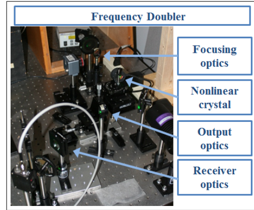
Fig. 10. Experimental setup for frequency doubler and associated optics.
