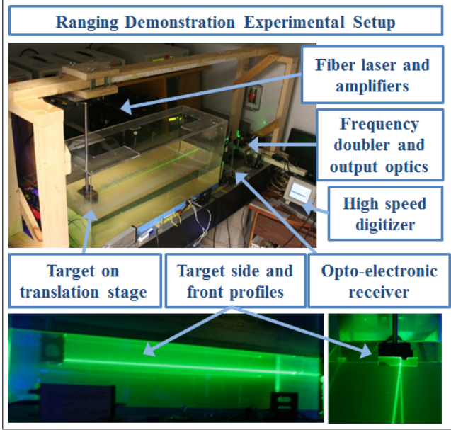
Fig. 12. Experimental setup of ranging demonstration. The target and stage allow translation over 120 cm round trip.
