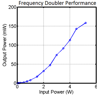
Fig. 11. Single-pass frequency doubling by a non-linear PPKTP crystal.
