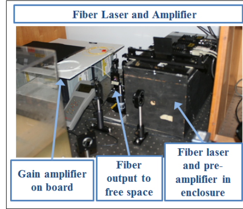
Fig. 6. Experimental setup for chaotic fiber laser and two fiber amplifier stages.
