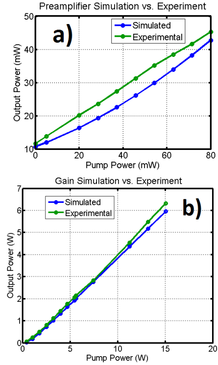
Fig. 9. Power amplification by two ytterbium-doped fiber amplifier stages. Top: Preamplifier output, experimental versus numerical simulation. Bottom: Gain amplifier output, experimental versus numerical simulation.
