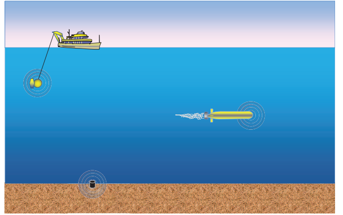
Fig. 1. Illustration of AUV-based geoacoustic inversions
