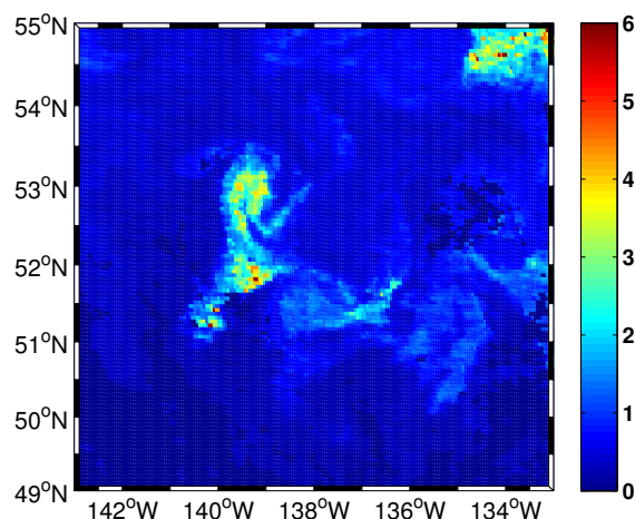
Fig. 20. Large scale composite of plankton bloom ( \mu\text{g/l} ) generated from satellite data.
