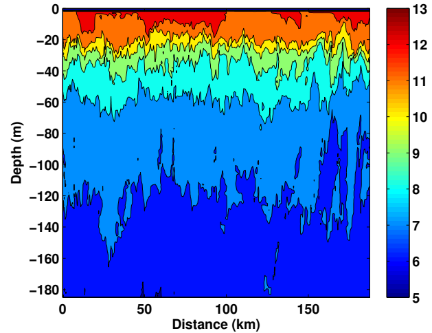
Fig. 13. Ascending temperature ( ^{\circ}\text{C} ) for the green portion of the long-range glider path.
