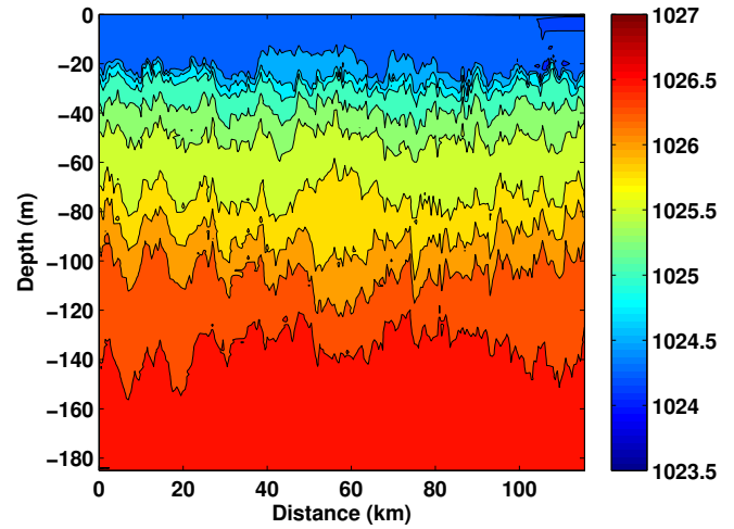
Fig. 17. Ascend density in \text{kg/m}^3 for water property change mission.
