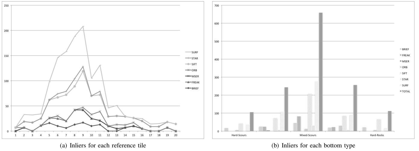
Fig. 4: Inliers from parallel test
