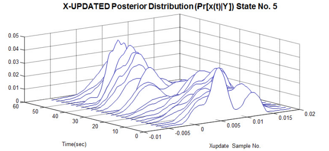
Fig. 4. PMF posterior estimation (mode 5) surface for Hudson Canyon 23-element array data (particle vs. time vs. probability).
