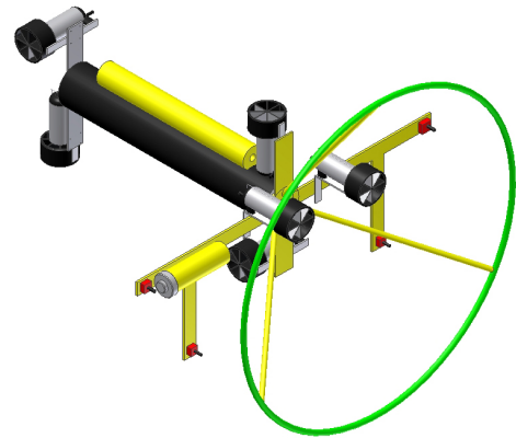
Fig. 1. AutoLARS CAD model
