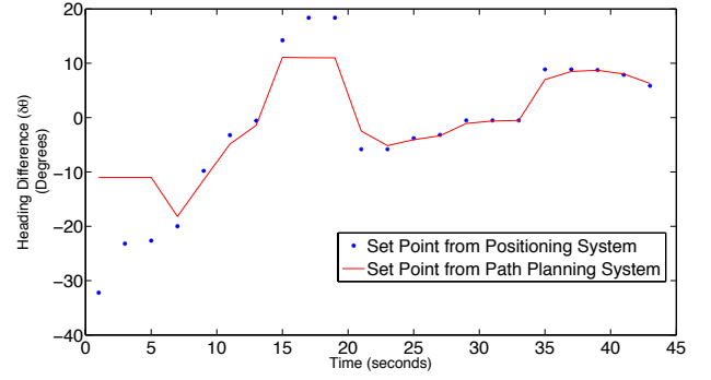
Fig. 11. Plot of azimuth from positioning system and path planning system
