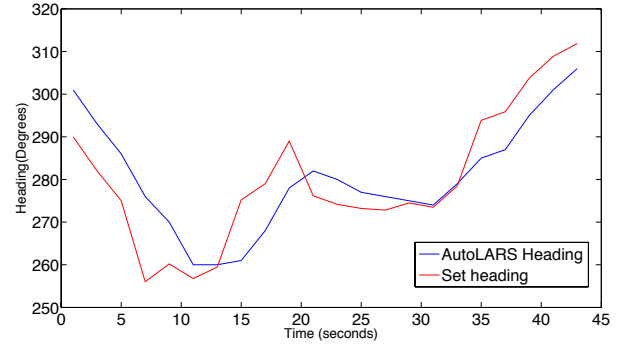
Fig. 12. The AutoLARS heading set point compensated to global frame comparison with actual heading
