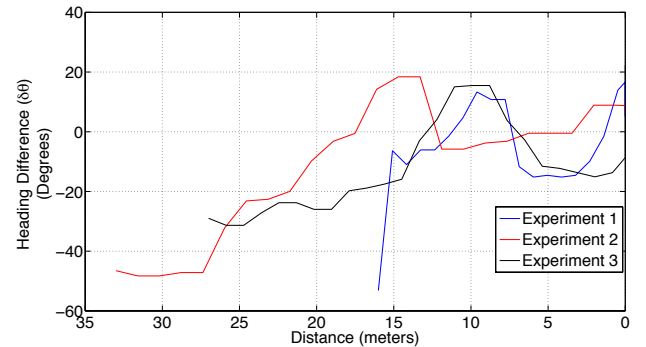
Fig. 13. Plot of Heading difference Vs Distance
