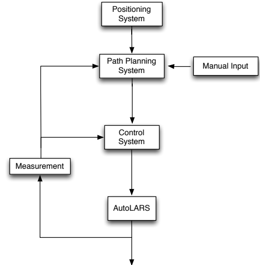
Fig. 4. A complete system configuration of AutoLARS
