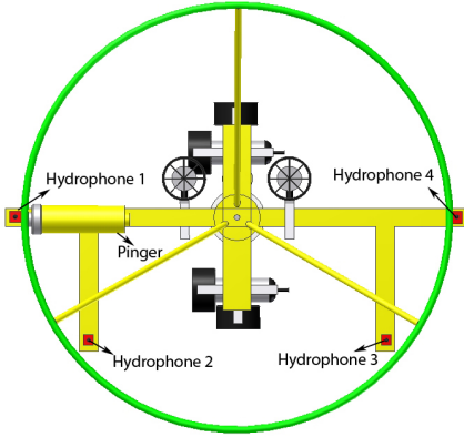
Fig. 2. Transducers and Pinger on AutoLARS
