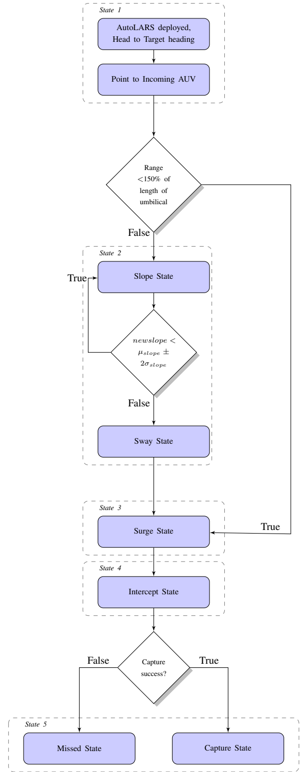
Fig. 8. A flow diagram detailing multiple states of the implemented path planning system
