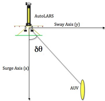
Fig. 10. Heading difference representation
