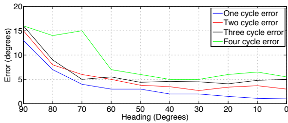
Fig. 3. Error vs angle plot when there is error on hydrophone 2
