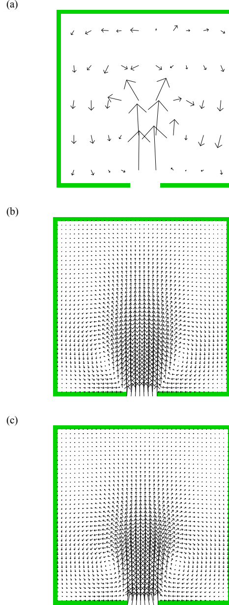
Fig. 2. Flow pattern in the harbour: observations (a), PML model (b) and k - \epsilon model (c).
