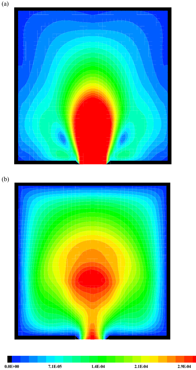
Fig. 4. Eddy viscosity ( \text{m}^2/\text{s} ) predicted by DIVAST with PML (a) and k-\epsilon model (b).
