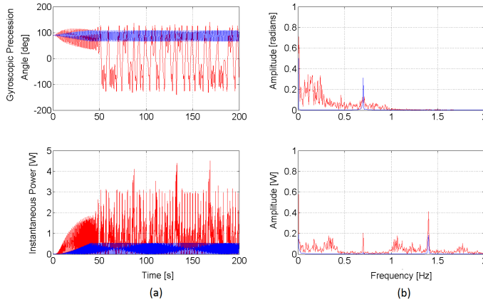
Fig. 10. Example gyroscopic precession and instantaneous power for a linear (blue, 15000rpm) and nonlinear (red, 30000rpm) response ((a) Time domain response (b) Frequency domain response)( \omega = 0.7\text{Hz} , B_g=0.2 )
