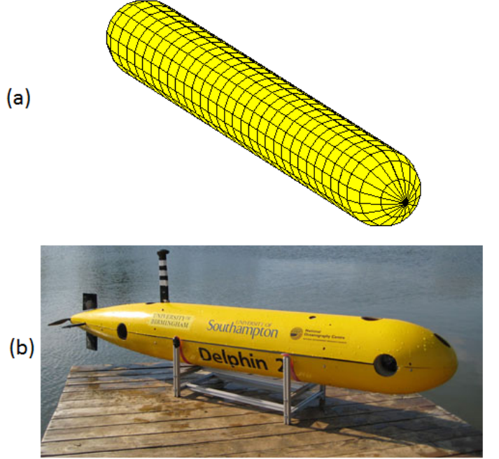
Fig. 4. (a) The simplified AUV model (b) the DELPHIN2 AUV
