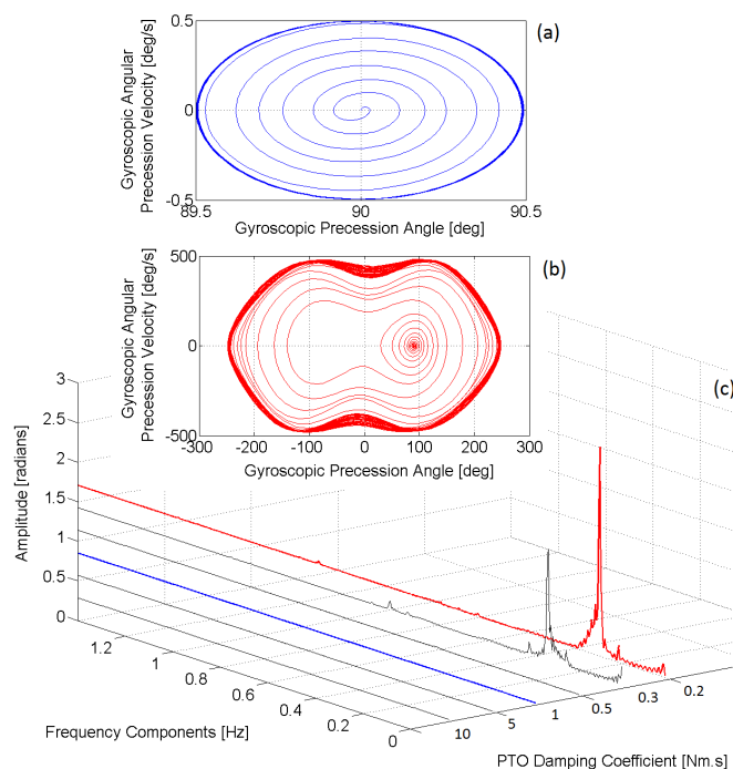
Fig. 12. Example low frequency gyroscopic precession responses ((a) Linear response (blue, B_g=1\text{Nm.s} ) (b) Predicted nonlinear response (red, B_g=0.2\text{Nm.s} ) (c) Frequency response over a range of damping coefficients ( B_g )) ( \omega=0.16\text{Hz} , 35000\text{rpm} )
