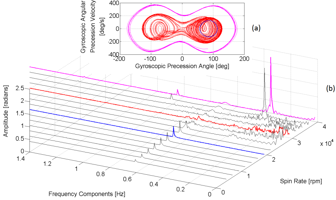
Fig. 9. Gyroscopic precession responses over a range of spin rates ((a) Example phase plots (magenta:40000rpm, red:30000rpm, blue:20000rpm)(b) Frequency response over a range of spin rates)( \omega=0.7\text{Hz} , B_g=0.3 )
