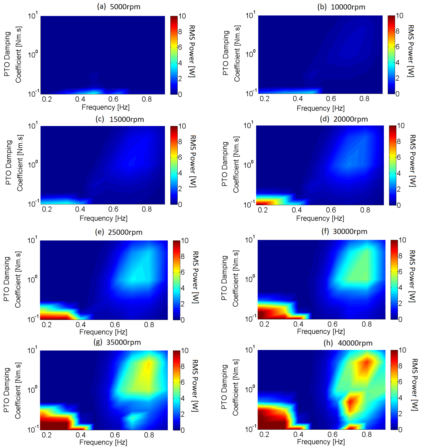
Fig. 11. Available rms power for the modelled 2m, 84kg cylindrical AUV in 0.1m wave amplitudes
