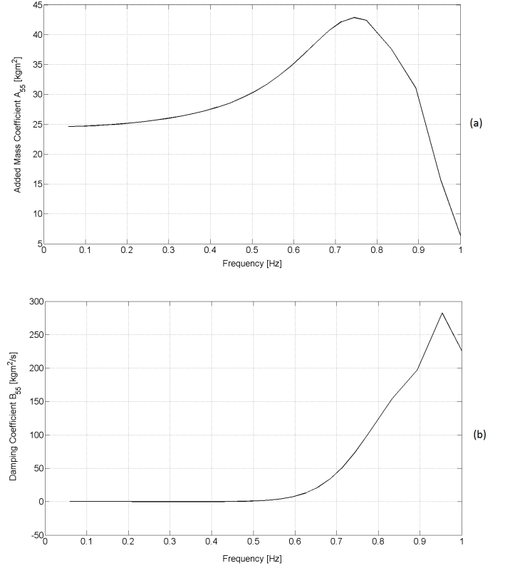
Fig. 6. Hydrodynamic coefficients ((a) Added mass A_{55} (b) Damping B_{55} )
