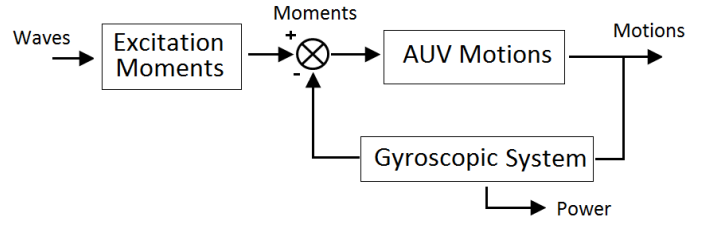
Fig. 3. Block diagram representation of the system
