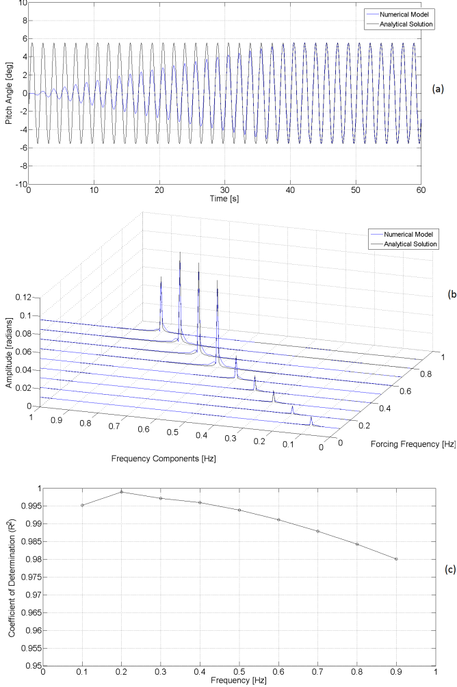
Fig. 7. Comparison of numerical and analytical solutions ((a): Example time history (frequency= 0.6Hz) (b): Frequency responses (c): Coefficient of determination ( R^2 ))(dt=0.05)
