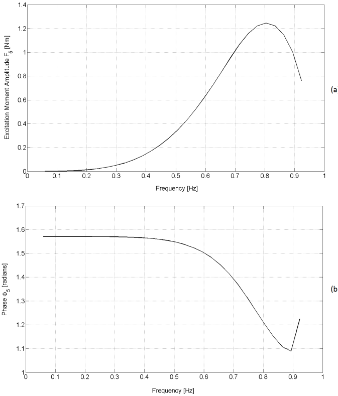
Fig. 5. Pitch excitation moments F_5 (a) and phases \Phi_5 (b) (wave amplitude of 0.1m)
